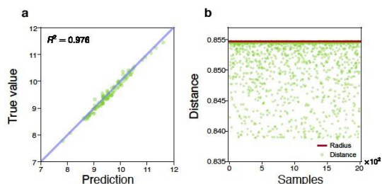
Figure 4: Stochastic simulations for Example 1.
