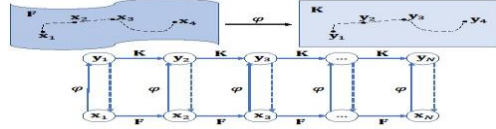
Figure 1: Schematic of Koopman operator theory. A measurement function \varphi maps system states \mathbf{x}_k into a high-dimensional space where measurements \mathbf{y}_k evolve linearly governed by Koopman operator \mathbf{K} , while the evolution operator of states \mathbf{x}_k is usually non-linear [32].
