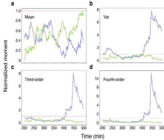
Figure 6: Sensitivity of moments against anomaly. The anomaly occurs at time t = 401 . All the moments are normalized for visual convenience, and the normalization methods are stated in Appendix 6.2. Moments of order higher or equal to 2 are sensitive to anomaly, while the mean value is not.
