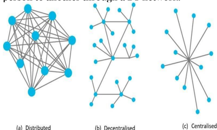
Figure 2: Illustration of nodes in a network showing the difference between a centralised, decentralised and distributed nodes. A decentralised, distributed network is fundamental to blockchain technology.
