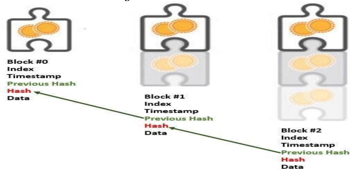
Figure 1: Representation of blocks in a blockchain, showing how the previous block is linked to the next block through the stored hash value
