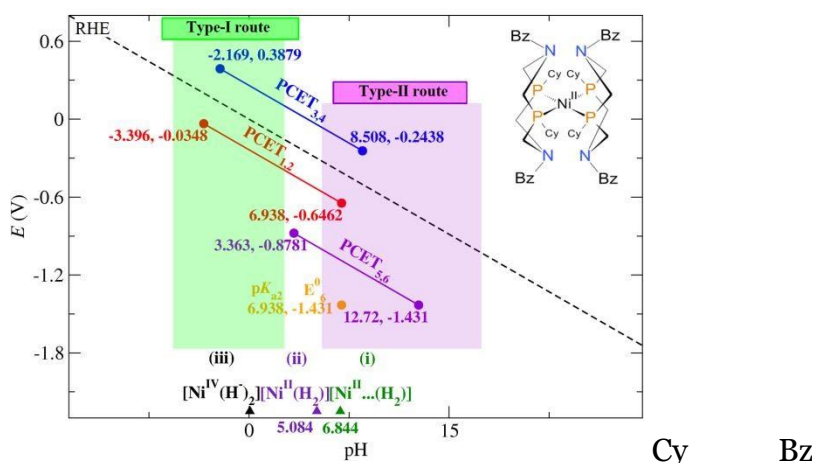
Fig. 14. Coupled Pourbaix diagram of model [\text{Ni}(\text{P}^{\text{Cy}}_2\text{N}^{\text{Bz}}_2)_2] . Intermediates involved in the Type-II \text{H}_2 bond cleaved pathway are shaded in purple, and intermediates involved in the Type-I \text{H}_2 bond cleaved pathway are shaded in green.
