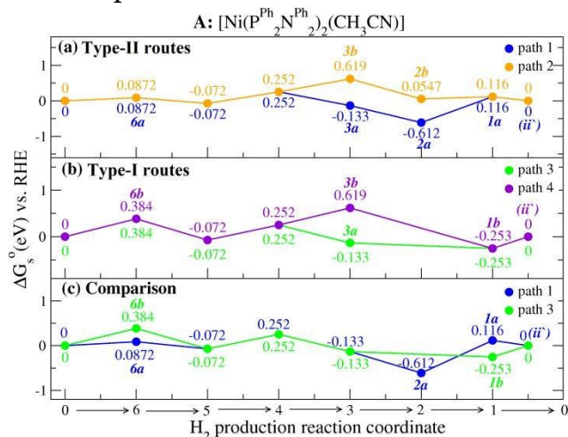
Fig. 8: Summary of mechanistic routes leading to \text{H}_2 production of
