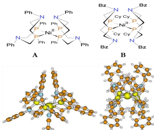
Fig. 1: Crystal structures from DuBois references are: (A) [\text{Ni}(\text{PPh}_2\text{NPh}_2)_2(\text{CH}_3\text{CN})](\text{BF}_4)_2 \text{PPh}_2\text{NPh}_2 = 1,3,5,7\text{-tetraphenyl-1,5-diaza-3,7-diphosphacyclooctane} , shown to work in the \text{H}_2 production direction; and (B) [\text{Ni}(\text{PCy}_2\text{NBz}_2)_2] shown to work in the \text{H}_2 oxidation direction.
