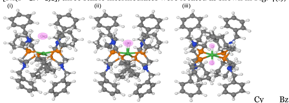
Fig. 4. Intermediates of the \text{H}_2 adduct to [\text{Ni}(\text{P}^{\text{Cy}}_2\text{N}^{\text{Bz}}_2)_2] model. (i) loosely bound dihydrogen [\text{Ni}^{\text{II}}\dots\text{H}_2]^{2+} ; (ii) strongly bound dihydrogen [\text{Ni}^{\text{II}}(\text{H}_2)]^{2+} ; and (iii) dihydride [\text{Ni}^{\text{IV}}(\text{H}^-)_2]^{2+} trans axial the plane of the metal center and phosphorous atoms.
