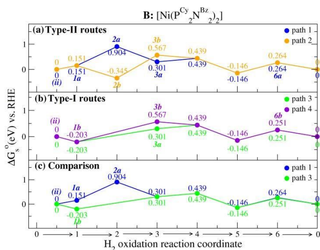
Fig. 10. Summary of mechanistic pathways leading to H 2 oxidation with the [Ni(PCy 2 N Bz ) 2 ] 2 model at conditions of pH = 0. Energy differences are taken with respect to the first point and normalized to the reversible hydrogen electrode (RHE).
