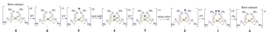
Fig. 9. Type-II \text{H}_2 bond cleaved path 1 for \text{H}_2 production of the [\text{Ni}(\text{PPh}_2\text{NPh}_2)_2(\text{CH}_3\text{CN})] model catalyst. The intermediates along this Path are 0 \square 6a \square 5 \square 4 \square 3a \square 2a \square 1a \square 0 .
