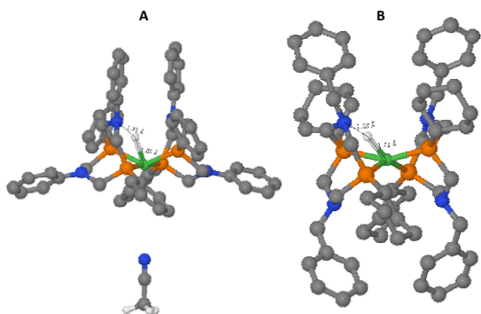
Fig. 7. Oxidative addition transition state, between intermediates 5 \rightarrow 4 , for compound A , [\text{Ni}(\text{P}^{\text{Ph}_2\text{N}^{\text{Ph}_2})_2(\text{CH}_3\text{CN})] model and compound B , [\text{Ni}(\text{P}^{\text{Cy}_2\text{N}^{\text{Bz}_2})_2] model.
