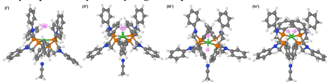
Fig. 5: Intermediates of the \text{H}_2 adduct to [\text{Ni}(\text{P}^{\text{Ph}}_2\text{N}^{\text{Ph}}_2)_2(\text{CH}_3\text{CN})] model. (i') loosely bound dihydrogen [\text{Ni}^{\text{II}}\dots\text{H}_2]^{2+} ; (ii') strongly bound dihydrogen [\text{Ni}^{\text{II}}(\text{H}_2)]^{2+} ; (iii') trans axial dihydride [\text{Ni}^{\text{IV}}(\text{H}^-)_2]^{2+} and (iv') [\text{Ni}^{\text{IV}}(\text{H}^-)_2]^{2+} dihydride intermediate.
