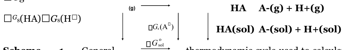
Scheme 1 General thermodynamic cycle used to calculate pK_a in acetonitrile solvent.
