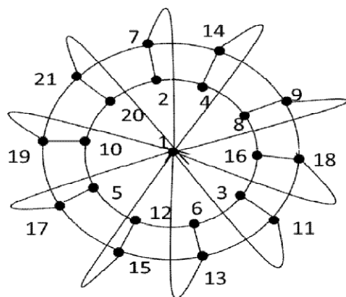
Figure: 6 Switching of apex vertex in
