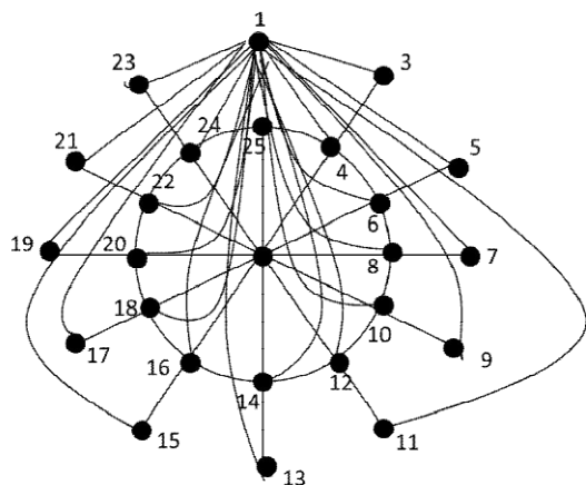
Figure 3: Switching of a pendant vertex of F_{l/2}
