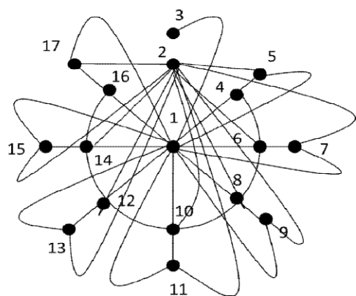
Figure 4: switching of a vertex v in F_{l/2}
