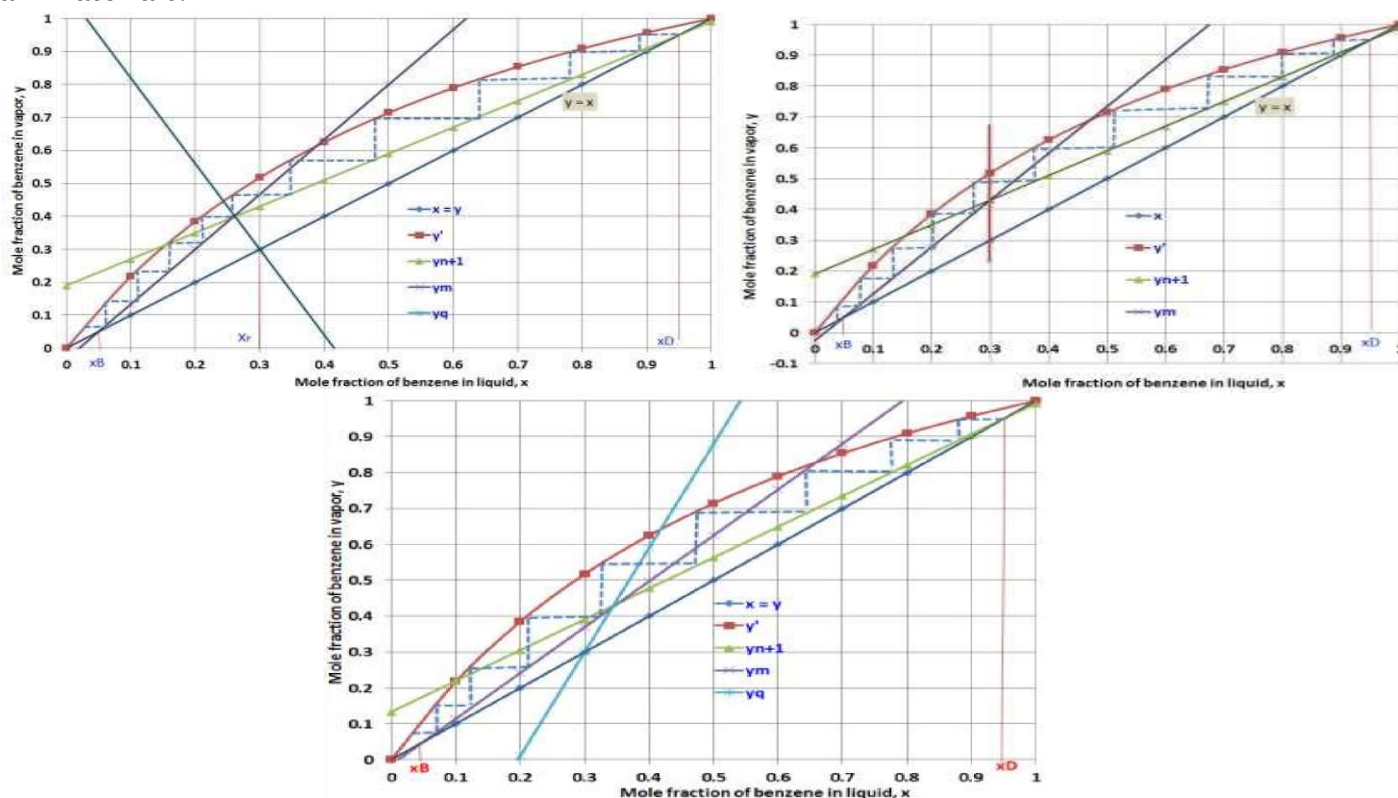
Figure 5. Variation of minimum number of stages, minimum reflux ratio and equilibrium number of stages with feed thermal conditions (VF, FBP, and SF) at a fixed feed composition x_F = 0.3 . conditions ( R = 4.0 ).
