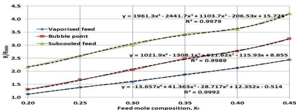
Figure 6. Effect of varying feed composition on minimum of reflux ratio for different feed thermal
