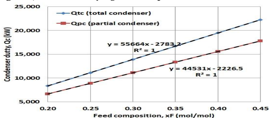
Figure 8. Effect of varying feed composition on the total and partial condenser duties.
