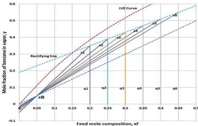
Figure 15. Loci of SOL and q lines for increasing composition of feed at its boiling point.
