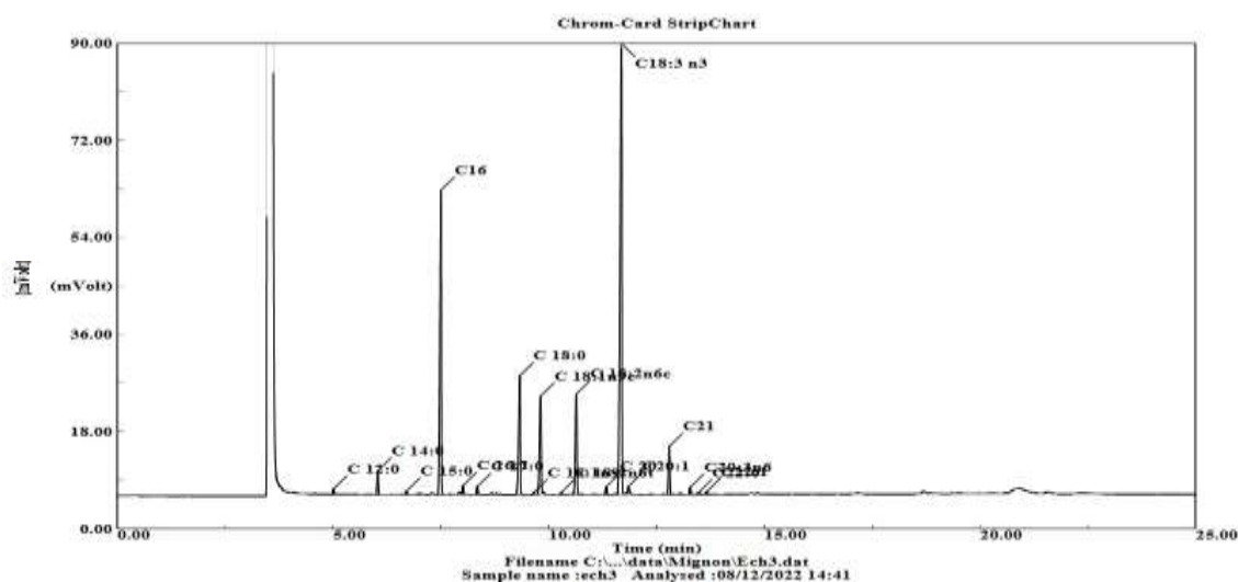
Figure 3. Chromatogram of the fatty acid profile of haplozana nigrolineata lipids.
