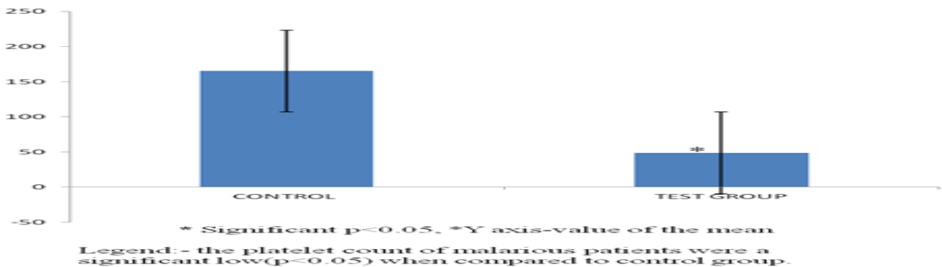
Figure 3: Shows difference in the Platelets count of malarious patients and control human.
